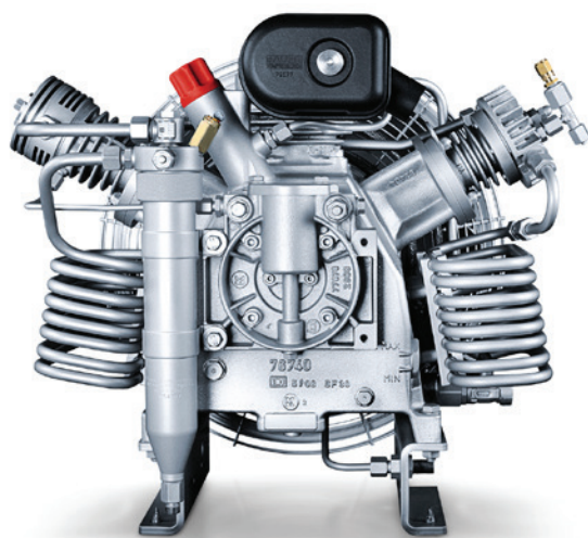
IK 120 Compressor Block (used in PE-TE, -HE, -MVE and -VE)
